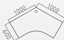
3-WAY CLUSTER WITH SINGLE DRAWER CONSUL
